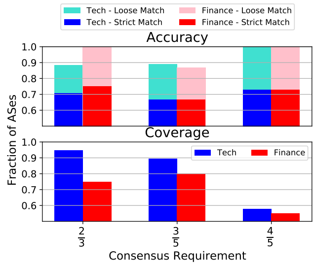
Figure 7: Amazon Mechanical Turk Consensus —Increasing the number of MTurks required for consensus (e.g., requiring 4/5 MTurks to agree instead of 2/3) increases accuracy by up to 12% and decreases coverage by up to 35%.
